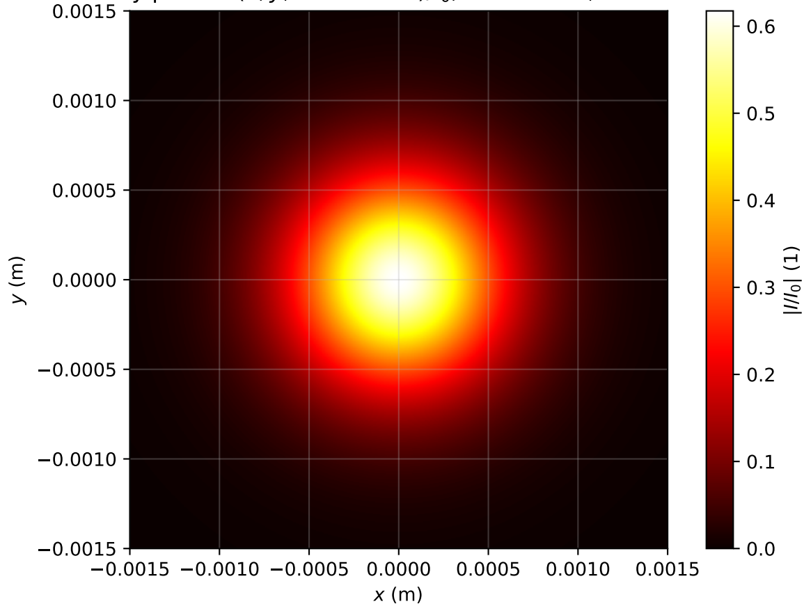
Intensity profile I(x, y, z = 3.264m)/I_0 , \text{Pin}=0.6\text{Pcr} , artificial time
